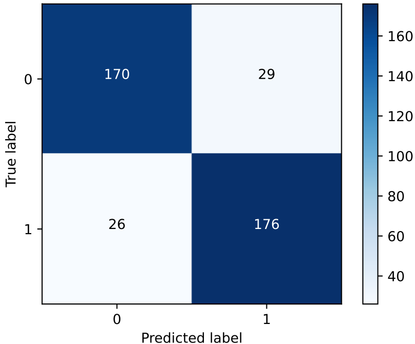
Confusion Matrix - GA_XGB (last fold)
