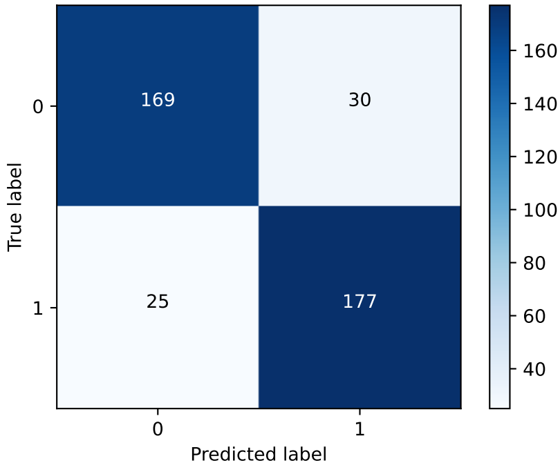
Confusion Matrix - LGB (last fold)
