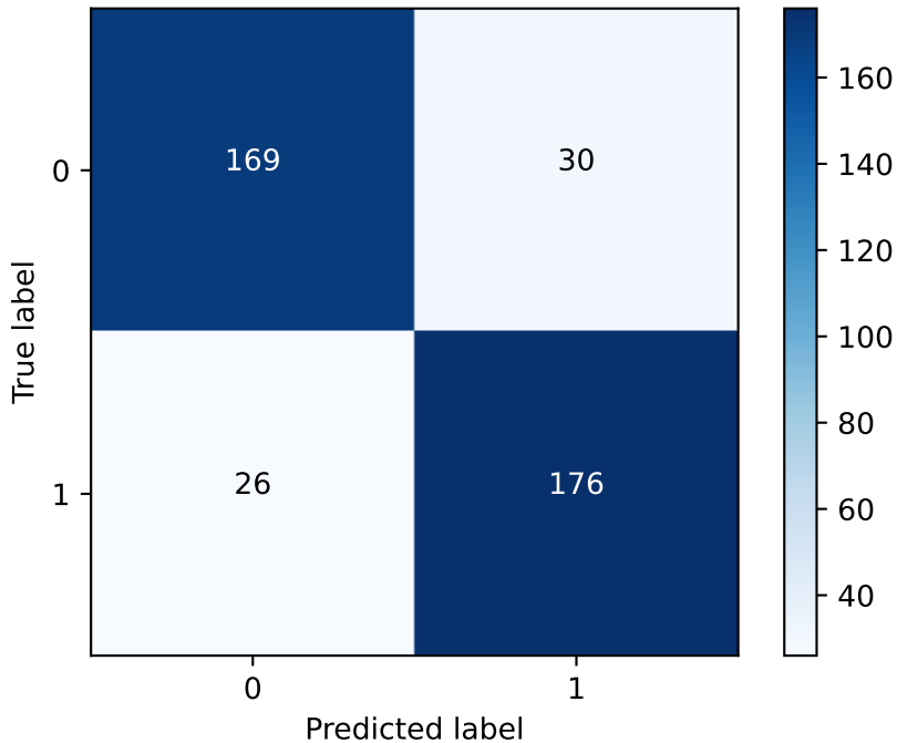
Confusion Matrix - XGB (last fold)
