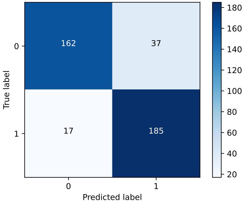
Confusion Matrix - STACKING (last fold)
