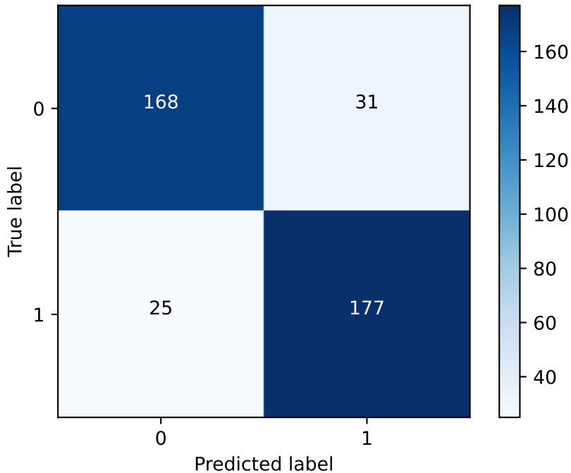
Confusion Matrix - VOTING (last fold)
