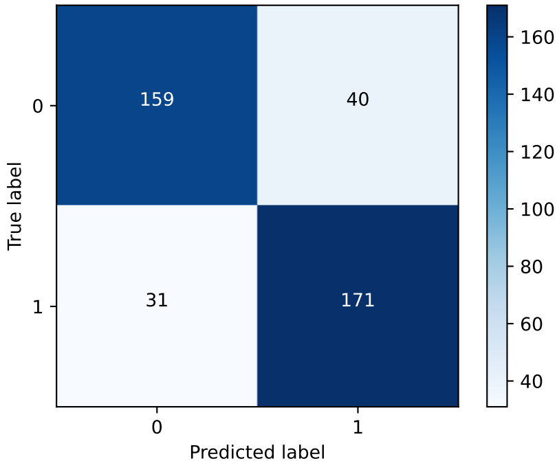
Confusion Matrix - BAGGING (last fold)
